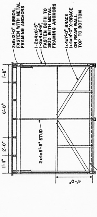
FRONT FRAMING
